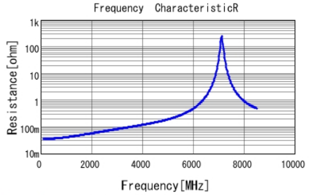
GQM2195C2E5R1DB12 R DCOV, 25degC
