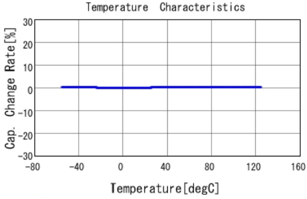
GQM2195C2E5R1DB12 C-Temp. capchange, DCOV, AC1Vrms
