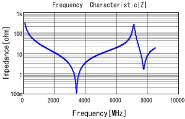
GQM2195C2E5R1DB12 |Z| DCOV, 25degC
