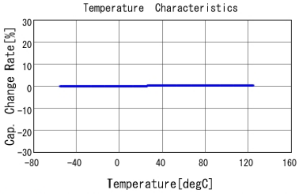
GRM21A5C2E820JW01 C-Temp. capchange, DCOV, AC1Vrms
