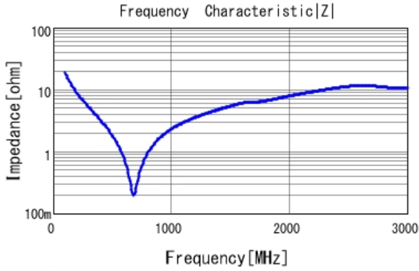
GRM21A5C2E820JW01 |Z| DCOV, 25degC
