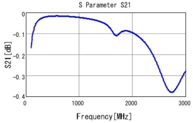
GRM21A5C2E820JW01 S21 DCOV, 25degC
