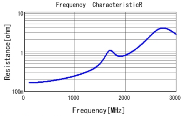
GRM21A5C2E820JW01 R DCOV, 25degC
