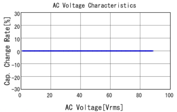
GRM21A5C2E820JW01 C-AC Voltage capchange, DCOV, 25
