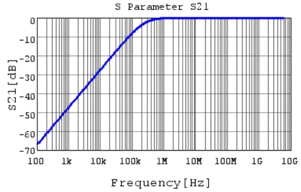
GRM033R61A682MA01 S21 DC0V,25degC
