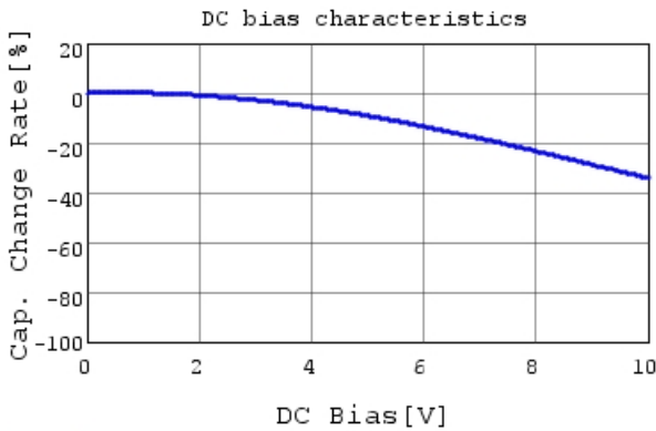
GRM033R61A682MA01 C-DC bias capchange, 25.0c
