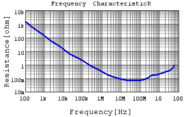
GRM033R61A682MA01 R DCOV, 25degC
