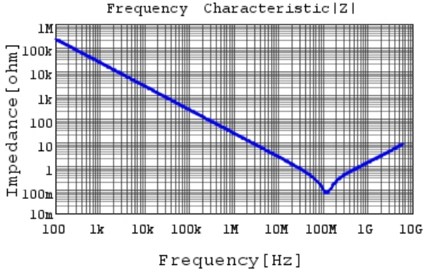
GRM033R61A682MA01 |Z| DCOV, 25degC
