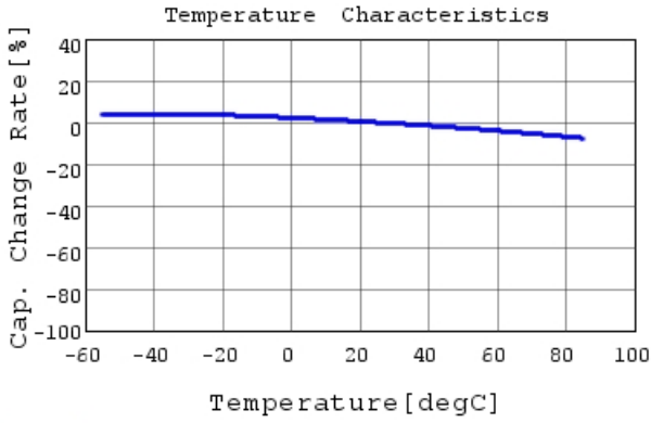
GRM033R61A682MA01 C-Temp. capchange, DC0.0V,
