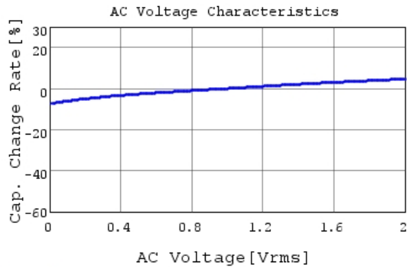
GRM033R61A682MA01 C-AC Voltage capchange, Dc
