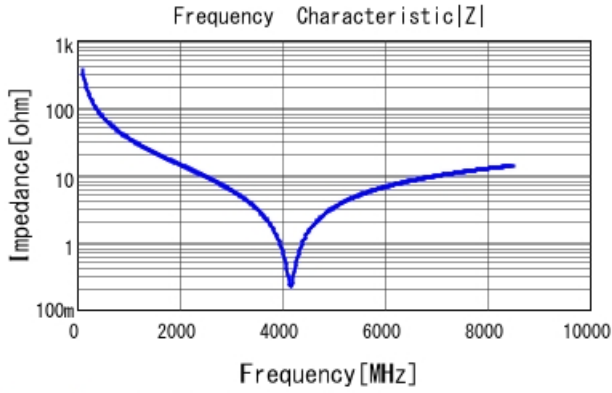
GJM1555C1H4R3CB01 |Z| DCOV, 25degC
