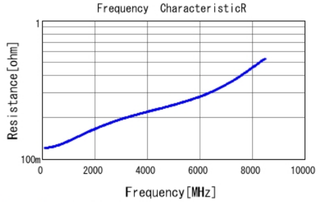
GJM1555C1H4R3CB01 R DCOV, 25degC
