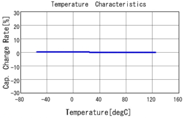
■ GCM0335C1H4R7CA16 C-Temp. capchange, DCOV, AC1Vrms
