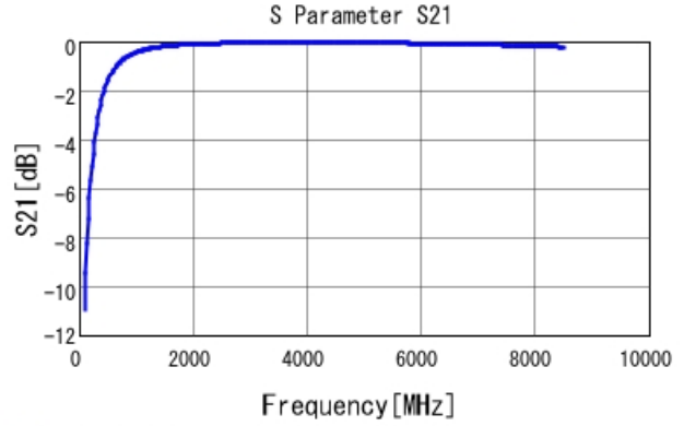
■ GCM0335C1H4R7CA16 S21 DCOV, 25degC
