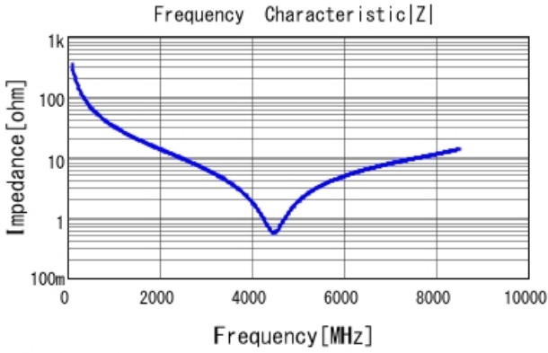
GCM0335C1H4R7CA16 |Z| DC0V, 25degC
