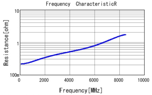
GCM0335C1H4R7CA16 R DC0V, 25degC
