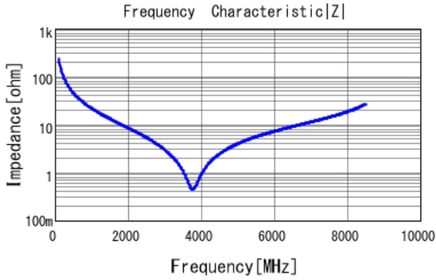
GCM0335C1E6R8CA16 |Z| DCOV, 25degC
