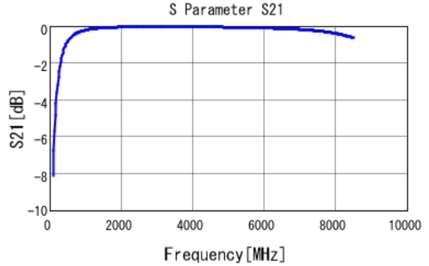
■ GCM0335C1E6R8CA16 S21 DCOV, 25degC
