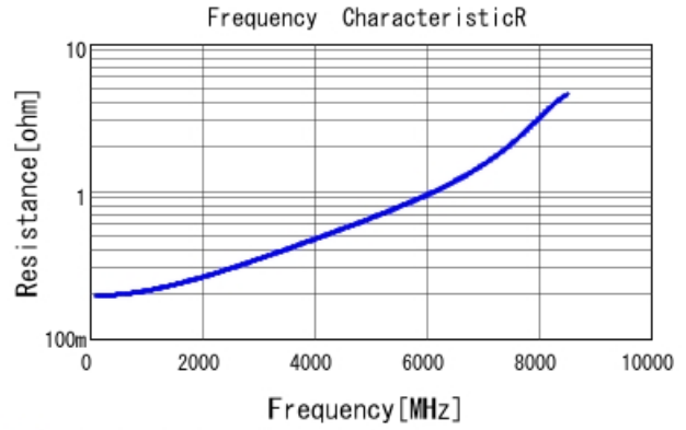
GCM0335C1E6R8CA16 R DCOV, 25degC
