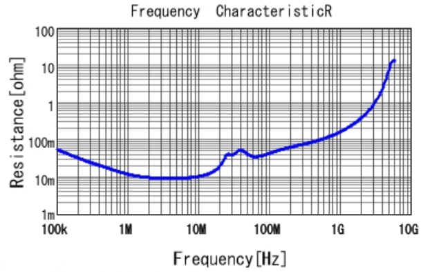
GRM219R71C334KA88 R DCOV, 25degC
