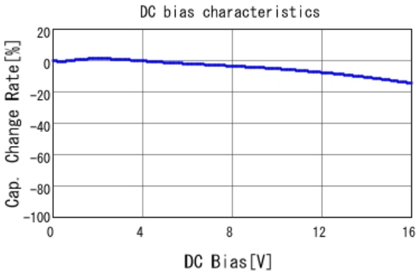
GRM219R71C334KA88 C-DC bias capchange, 25.0degC, A
