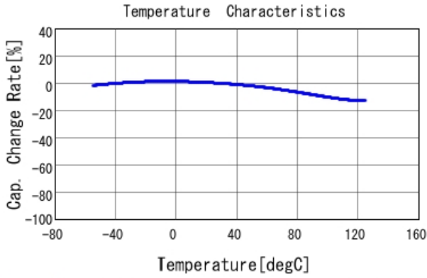
GRM219R71C334KA88 C-Temp. capchange, DC0.0V, AC1.C
