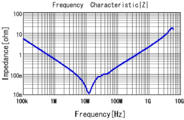
GRM219R71C334KA88 |Z| DCOV, 25degC
