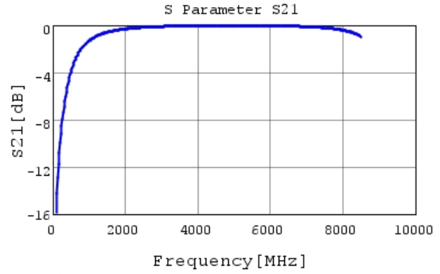
GCQ1555C1H2R6CB01 S21 DCOV, 25degC
