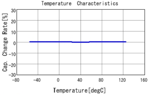
GRM1555C2A4R5BA01 C-Temp. capchange, DC0V, AC1Vrms
