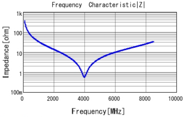
GRM1555C2A4R5BA01 |Z| DCOV, 25degC
