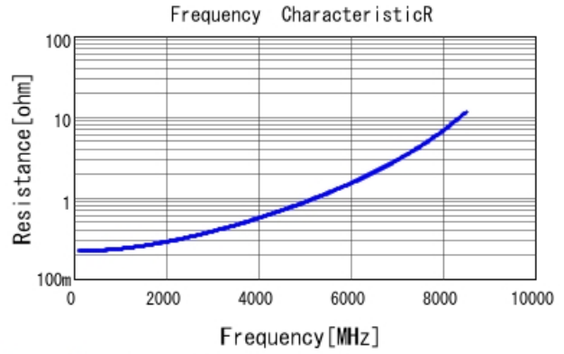
GRM1555C2A4R5BA01 R DCOV, 25degC
