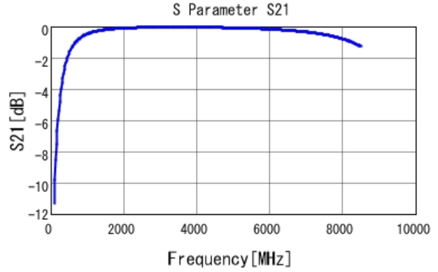
GRM1555C2A4R5BA01 S21 DC0V, 25degC
