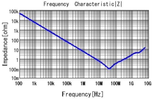
GCJ219R72A333KA01 |Z| DCOV, 25degC
