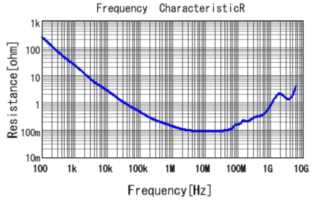
GCJ219R72A333KA01 R DCOV, 25degC
