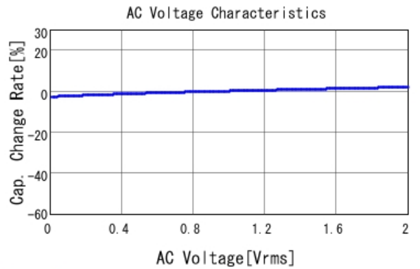
GCJ219R72A333KA01 C-AC Voltage capchange, DCOV, 25
