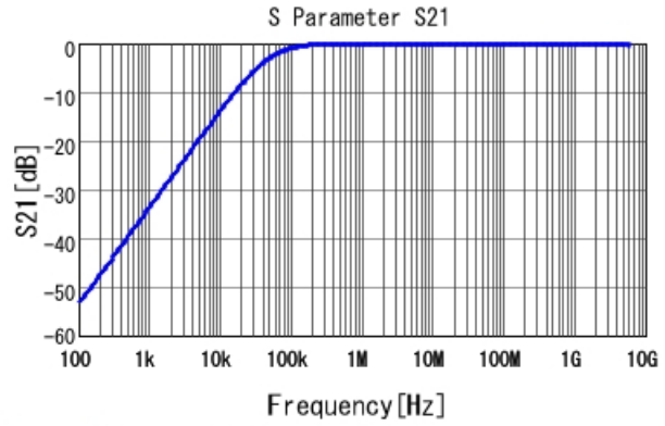
GCJ219R72A333KA01 S21 DC0V, 25degC
