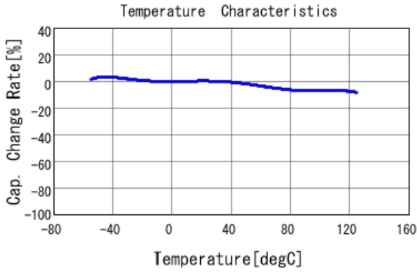
GCJ219R72A333KA01 C-Temp. capchange, DC0.0V, AC1.C
