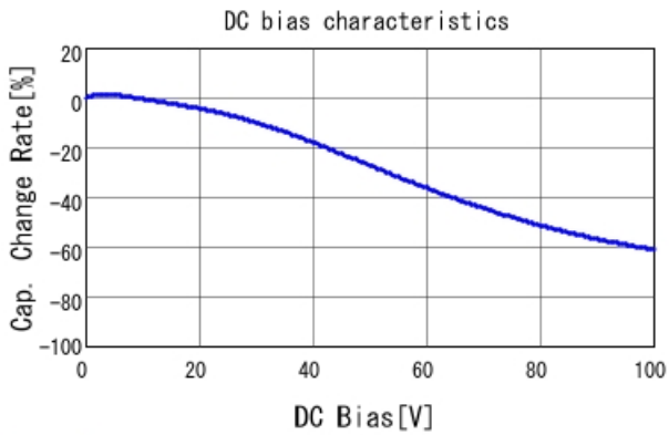
GCJ219R72A333KA01 C-DC bias capchange, 25.0degC, A
