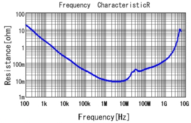
GRM219R71E474MA88 R DCOV, 25degC
