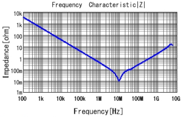
GRM219R71E474MA88 |Z| DCOV, 25degC
