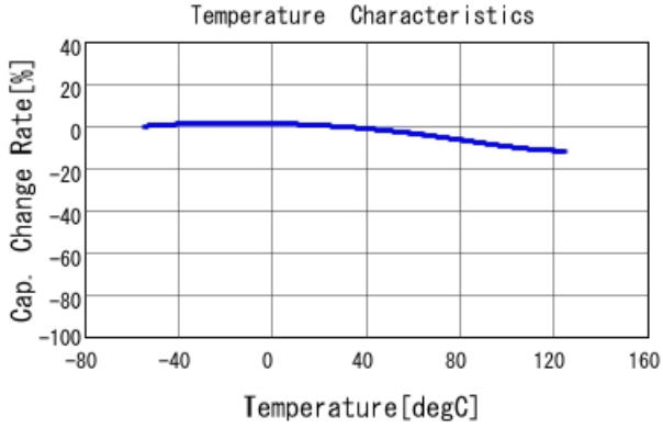
GRM219R71E474MA88 C-Temp. capchange, DC0.0V, AC1.C
