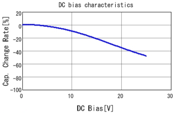
GRM219R71E474MA88 C-DC bias capchange, 25.0degC, A
