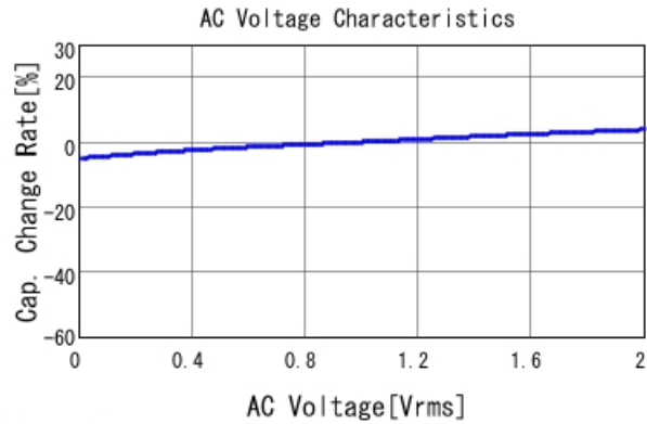
GRM219R71E474MA88 C-AC Voltage capchange, DCOV, 25
