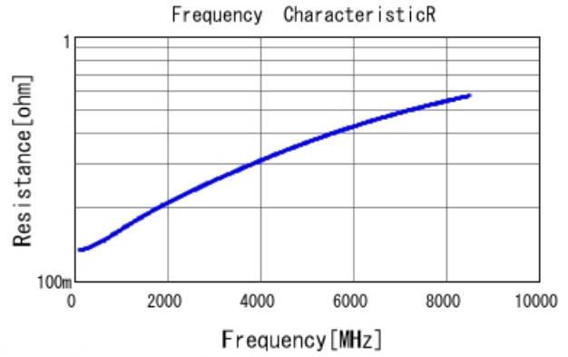
GRM0225C1E8R9DA03 R DCOV, 25degC
