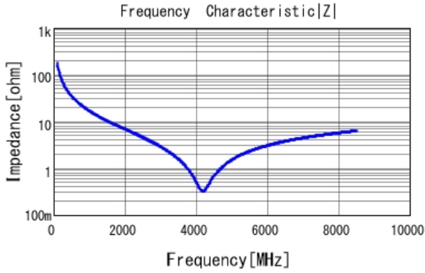
GRM0225C1E8R9DA03 |Z| DCOV, 25degC
