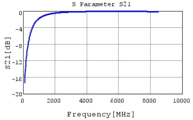
GRM0335C1H2R2BA01 S21 DCOV, 25degC
