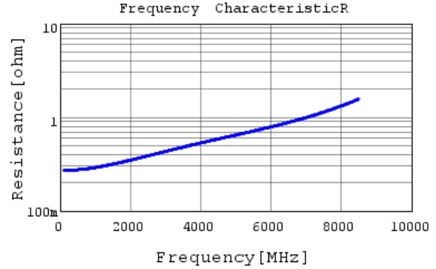
GRM0335C1H2R2BA01 R DCOV, 25degC
