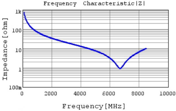
GRM0335C1H2R2BA01 |Z| DCOV, 25degC
