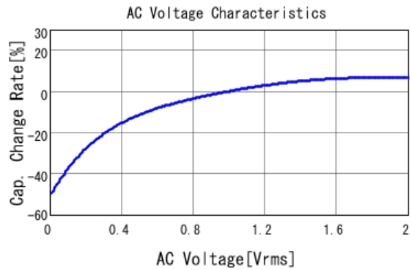
GRM219R61C106MA73 C-AC Voltage capchange, DCOV, 25
