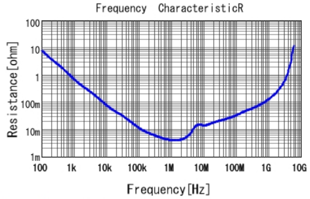
GRM219R61C106MA73 R DCOV, 25degC
