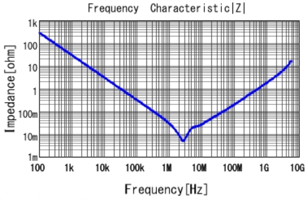
GRM219R61C106MA73 |Z| DCOV, 25degC
