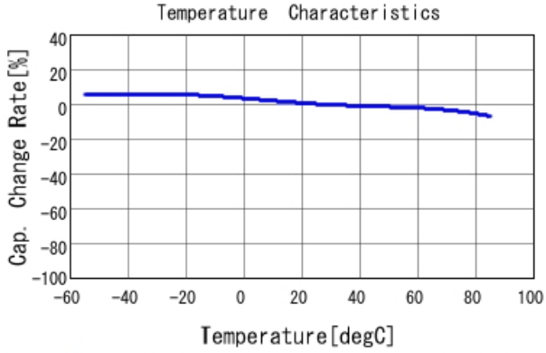
GRM219R61C106MA73 C-Temp. capchange, DC0.0V, AC1.C
