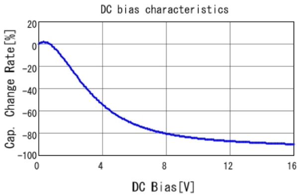
GRM219R61C106MA73 C-DC bias capchange, 25.0degC, A
