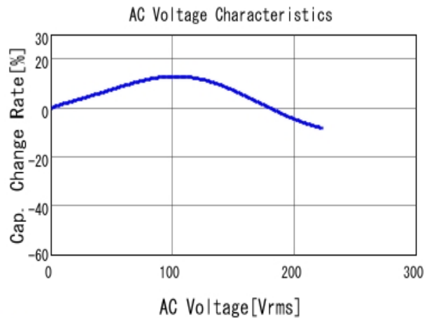
■ GCJ31CR72J153KXJ3 C-AC Voltage capchange, DC0V, 25.0d
