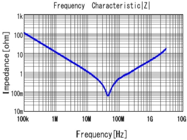
■ GCJ31CR72J153KXJ3 |Z| DC0V, 25degC
