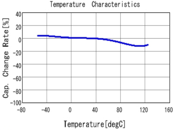
■ GCJ31CR72J153KXJ3 C-Temp. capchange, DCOV, AC1Vrms
