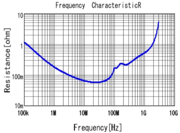
■ GCJ31CR72J153KXJ3 R DC0V, 25degC
