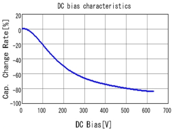
■ GCJ31CR72J153KXJ3 C-DC bias capchange, 25.0degC, AC1V
