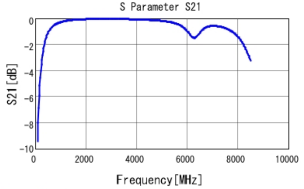
GRM1885C2A5R7WA01 S21 DCOV, 25degC
