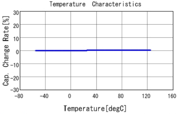
GRM1885C2A5R7WA01 C-Temp. capchange, DCOV, AC1Vrms
