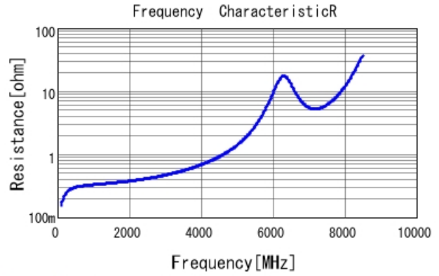
GRM1885C2A5R7WA01 R DCOV, 25degC
