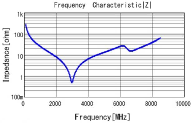
GRM1885C2A5R7WA01 |Z| DCOV, 25degC
