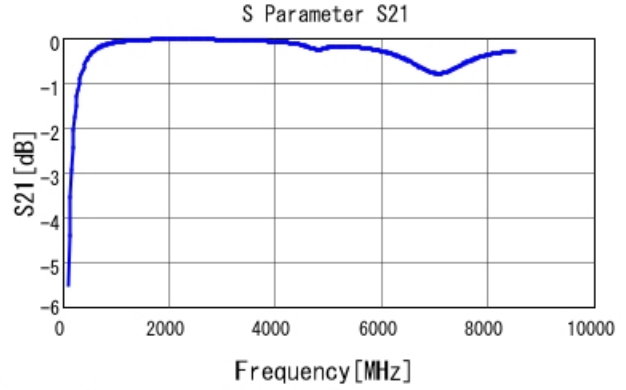
GRM1885C2A9R9DA01 S21 DCOV, 25degC
