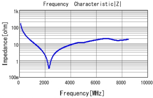
GRM1885C2A9R9DA01 |Z| DCOV, 25degC
