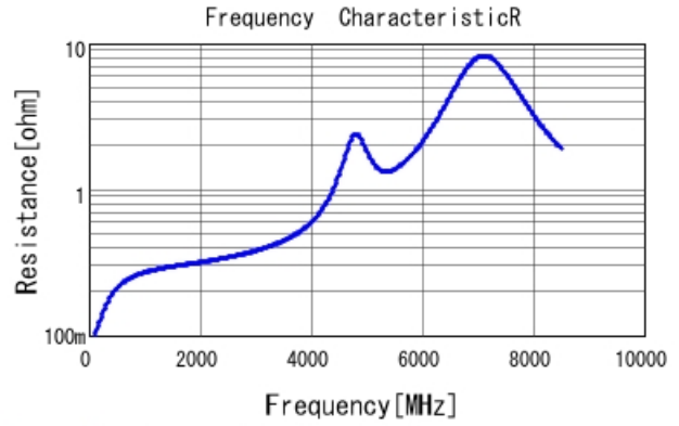
GRM1885C2A9R9DA01 R DCOV, 25degC
