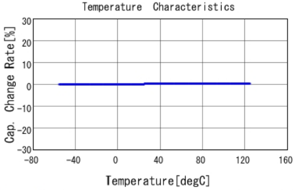
GRM1885C2A9R9DA01 C-Temp. capchange, DCOV, AC1Vrms
