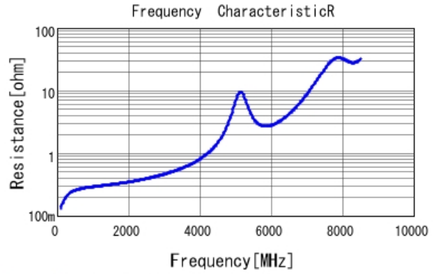
GRM1885C1H8R5DA01 R DCOV, 25degC
