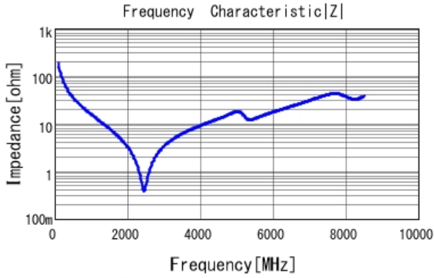
GRM1885C1H8R5DA01 |Z| DCOV, 25degC
