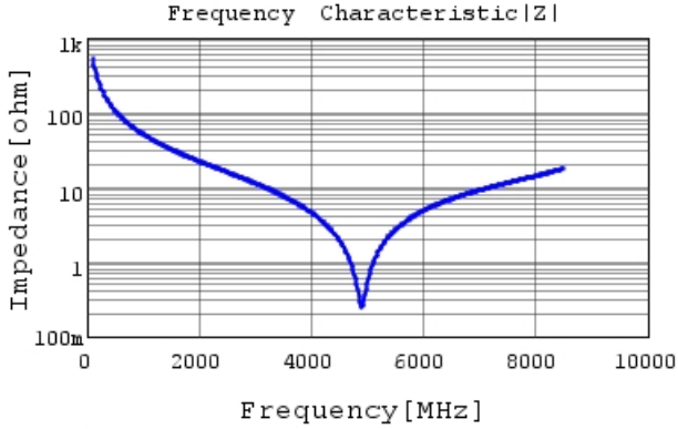
GCQ1555C1H3R0BB01 |Z| DC0V, 25degC
