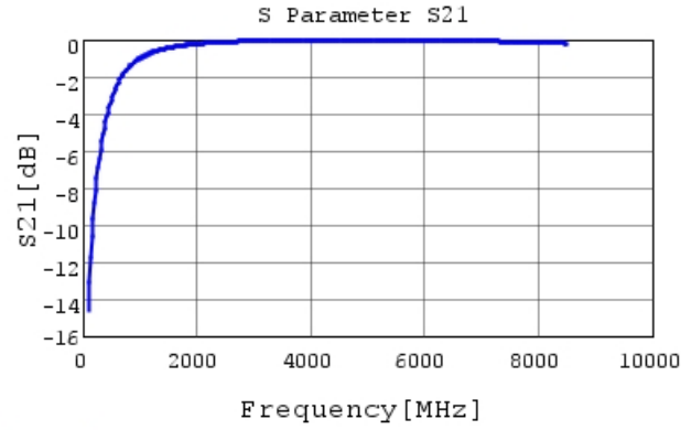
GCQ1555C1H3R0BB01 S21 DCOV, 25degC
