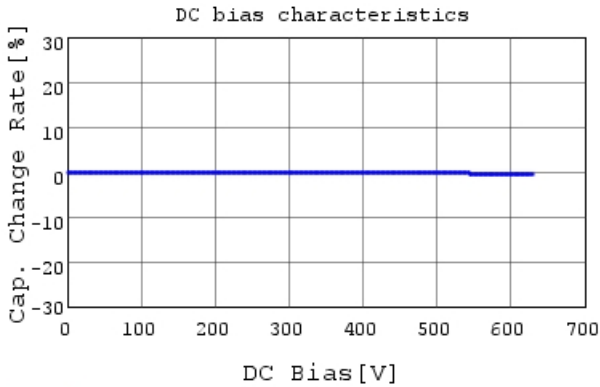
GCM31A5C2J102JX01 C-DC bias capchange, 25.0c
