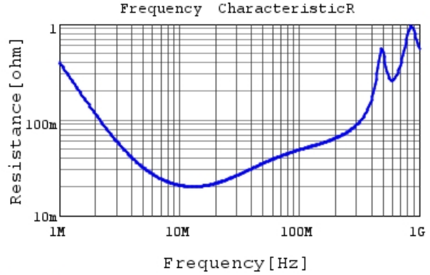
GCM31A5C2J102JX01 R DC0V, 25degC
