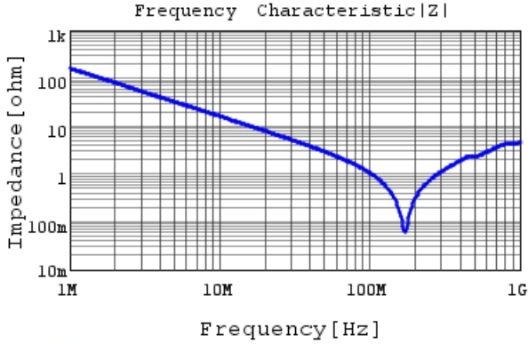
GCM31A5C2J102JX01 |Z| DC0V, 25degC
