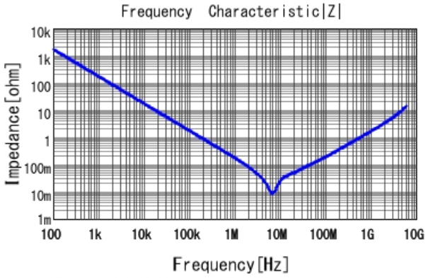
GRM188B10J105KA01 |Z| DCOV, 20degC
