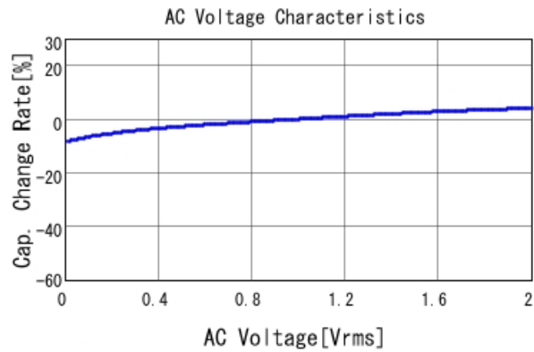
GRM188B10J105KA01 C-AC Voltage capchange, DCOV, 2C
