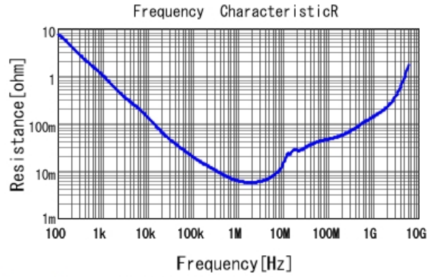
GRM188B10J105KA01 R DCOV, 20degC
