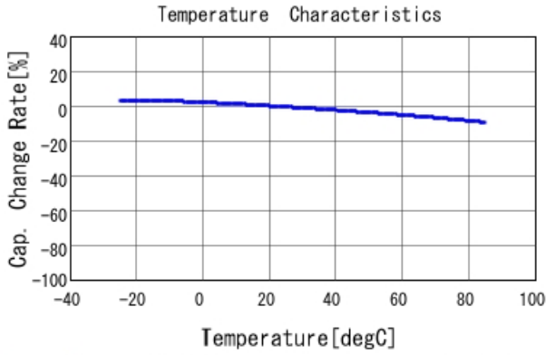
GRM188B10J105KA01 C-Temp. capchange, DC0.0V, AC1.C
