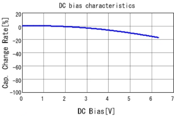
GRM188B10J105KA01 C-DC bias capchange, 20.0degC, A
