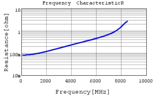
GCQ1555C1H7R2CB01 R DC0V, 25degC
