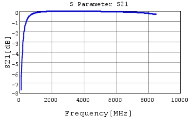
GCQ1555C1H7R2CB01 S21 DCOV, 25degC
