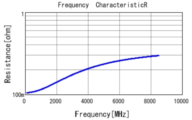
GJM0335C1E6R6BB01 R DCOV, 25degC
