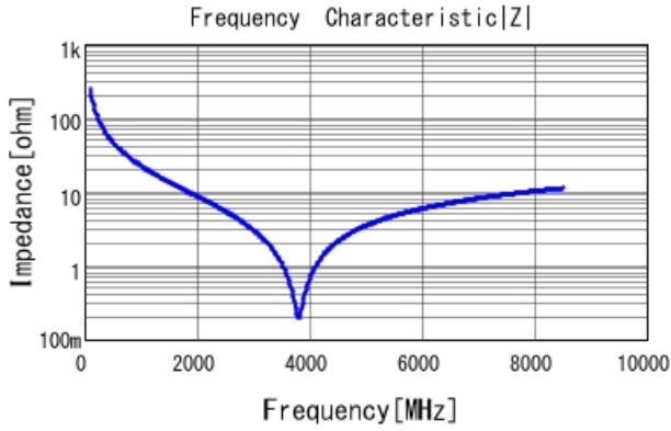
GJM0335C1E6R6BB01 |Z| DCOV, 25degC
