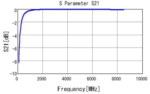
GJM0335C1E6R6BB01 S21 DCOV, 25degC
