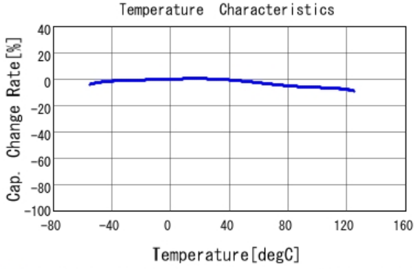
■ GCD188R71H562MA01 C-Temp. capchange, DCO. 0V, AC1. 0V rm
