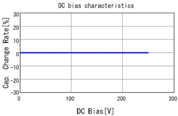
GQM1875C2E470GB12 C-DC bias capchange, 25.0degC, A
