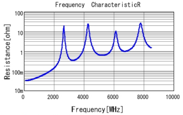
GQM1875C2E470GB12 R DCOV, 25degC
