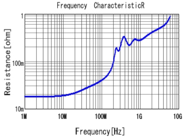
■ GRM1857U1H472JA44 R DCOV, 25degC
