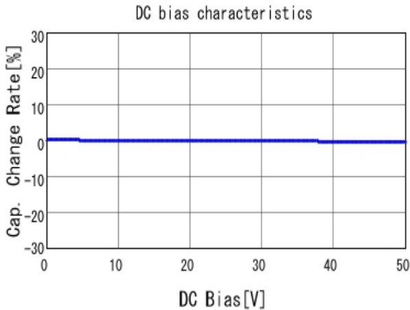
■ GRM1857U1H472JA44 C-DC bias capchange, 25.0degC, AC1V
