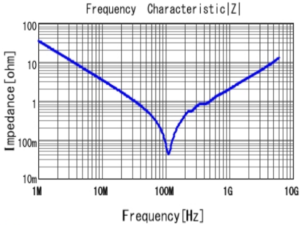
■ GRM1857U1H472JA44 |Z| DCOV, 25degC
