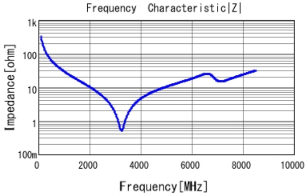
GRM1885C2A4R9WA01 |Z| DCOV, 25degC
