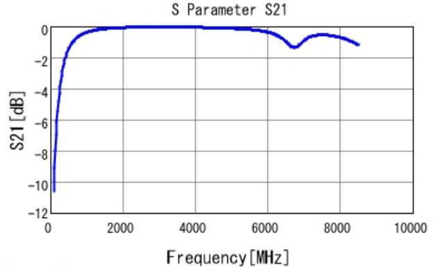
GRM1885C2A4R9WA01 S21 DCOV, 25degC
