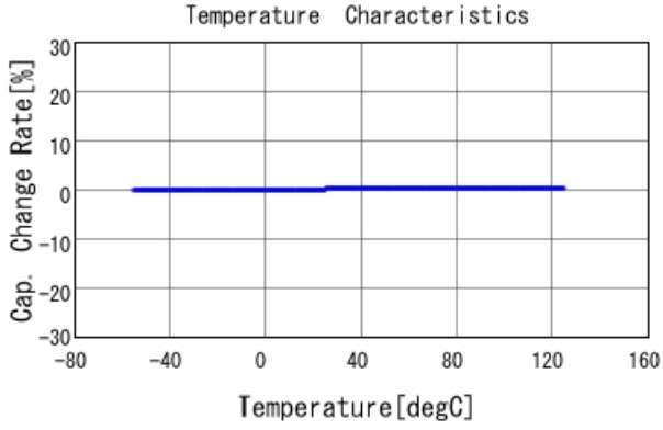
GRM1885C2A4R9WA01 C-Temp. capchange, DCOV, AC1Vrms
