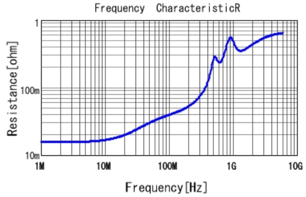
GCM2165C1H152JA16 R DCOV, 25degC
