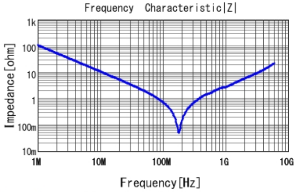
GCM2165C1H152JA16 |Z| DCOV, 25degC
