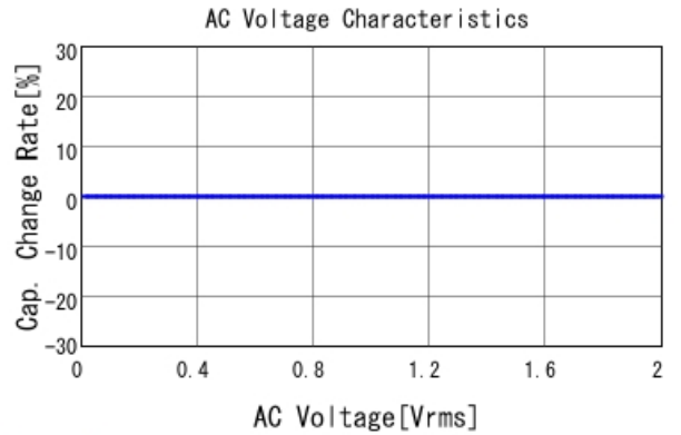
GCM2165C1H152JA16 C-AC Voltage capchange, DCOV, 25
