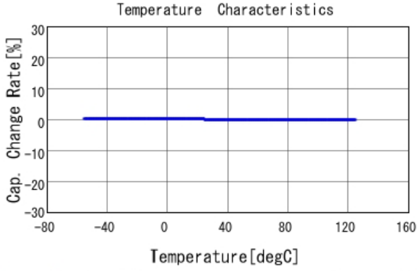
GCM2165C1H152JA16 C-Temp. capchange, DCOV, AC1Vrms
