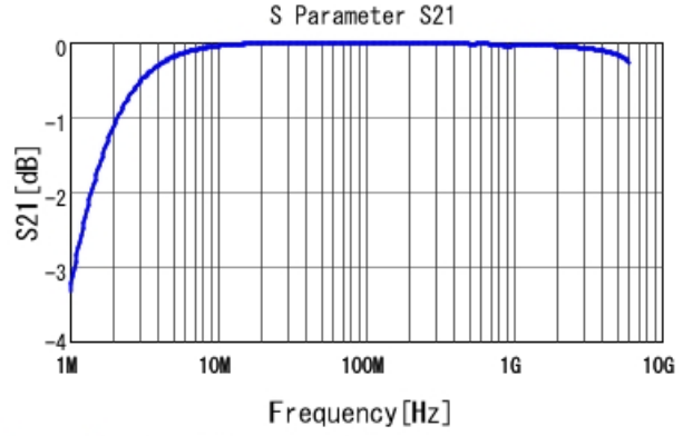
GCM2165C1H152JA16 S21 DCOV, 25degC
