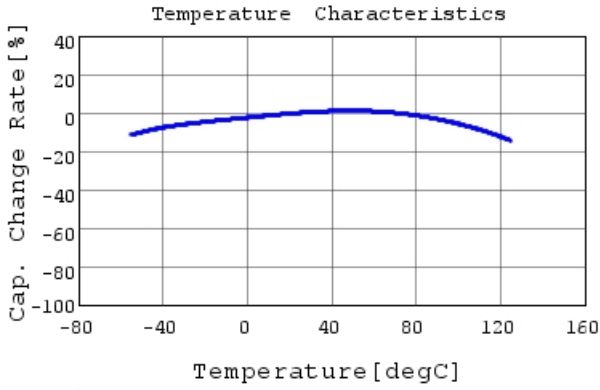
GCM21BR71E225KA73 C-Temp. capchange, DC0.0V,
