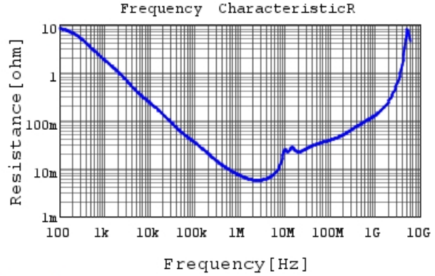
GCM21BR71E225KA73 R DC0V, 25degC
