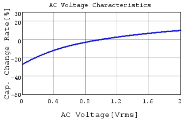
GCM21BR71E225KA73 C-AC Voltage capchange, DC
