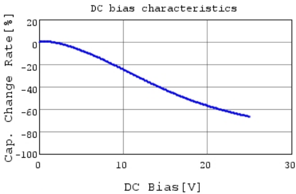
GCM21BR71E225KA73 C-DC bias capchange, 25.0c
