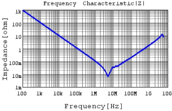
GCM21BR71E225KA73 |Z| DC0V, 25degC
