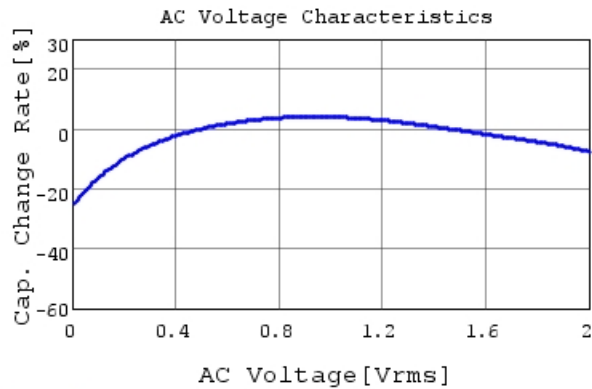
GRM188C80G226ME15 C-AC Voltage capchange, DC
