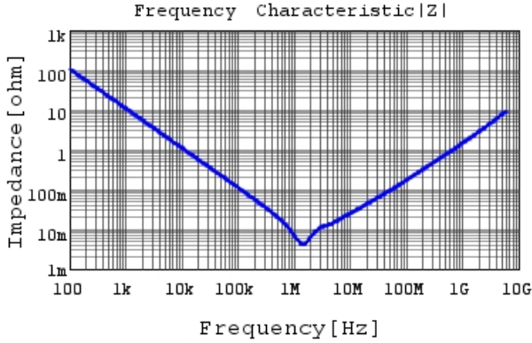
GRM188C80G226ME15 |Z| DCOV, 25degC
