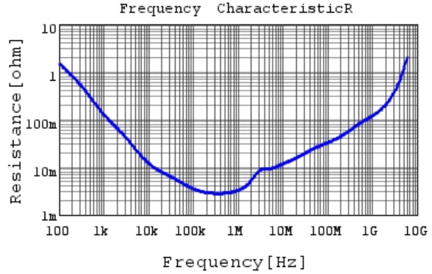
GRM188C80G226ME15 R DCOV, 25degC
