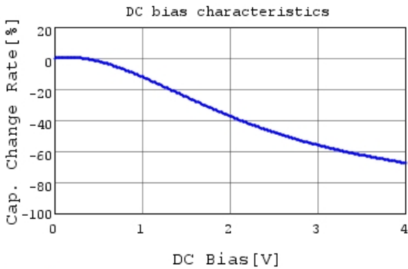
GRM188C80G226ME15 C-DC bias capchange, 25.0c
