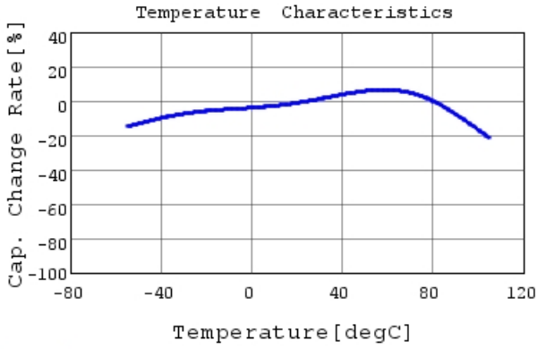
GRM188C80G226ME15 C-Temp. capchange, DC0.0V,
