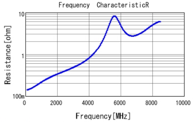
GRM1555C2A100JA01 R DCOV, 25degC
