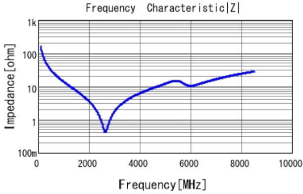
GRM1555C2A100JA01 |Z| DCOV, 25degC
