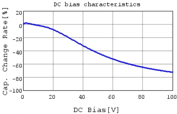
RCER72A223K0K1H03B C-DC bias capchange, 25.0
