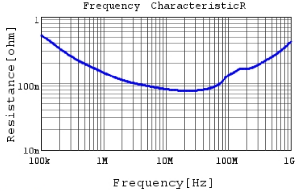
RCER72A223K0K1H03B R DCOV, 25degC
