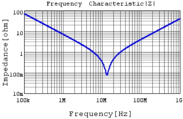
RCER72A223K0K1H03B |Z| DCOV, 25degC
