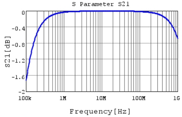
RCER72A223K0K1H03B S21 DC0V, 25degC
