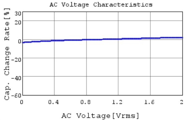
RCER72A223K0K1H03B C-AC Voltage capchange, I
