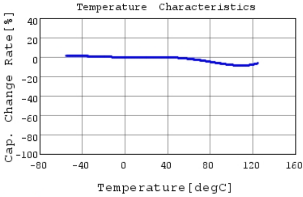
RCER72A223K0K1H03B C-Temp. capchange, DC0.0V
