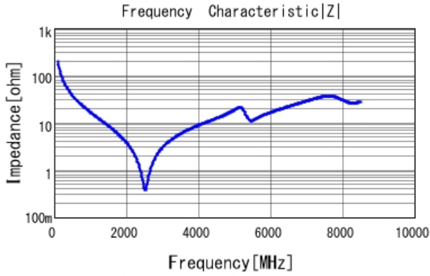
GRM1885C1H8R0DA01 |Z| DCOV, 25degC
