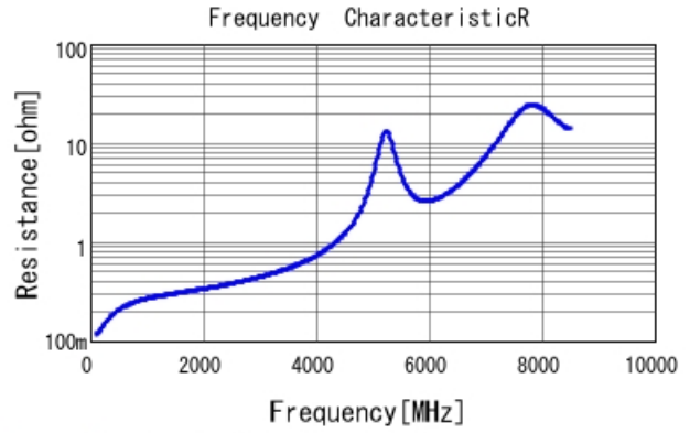
GRM1885C1H8R0DA01 R DCOV, 25degC
