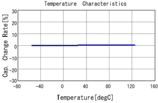
GRM1885C1H8R0DA01 C-Temp. capchange, DCOV, AC1Vrms
