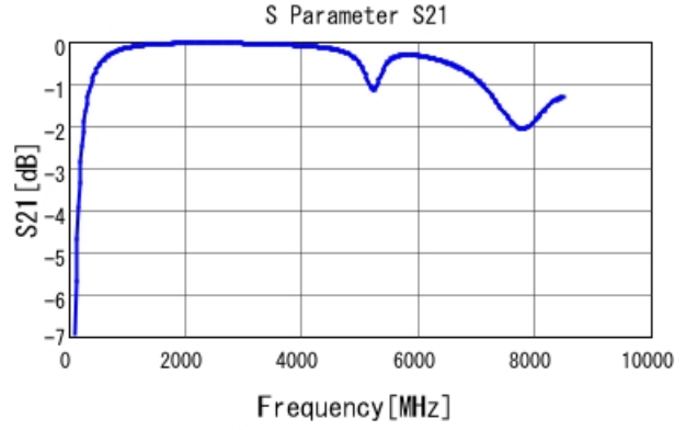
GRM1885C1H8R0DA01 S21 DCOV, 25degC
