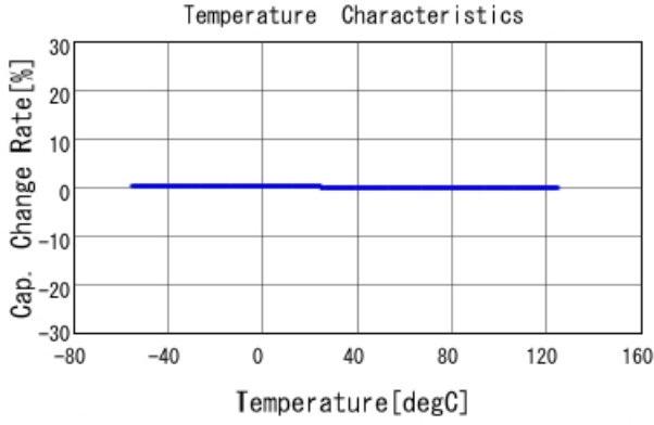
GRM0335C1H9R5CA01 C-Temp. capchange, DC0V, AC1Vrms
