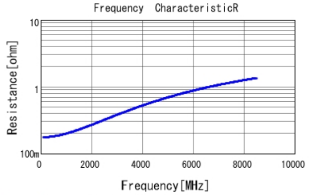
GRM0335C1H9R5CA01 R DCOV, 25degC
