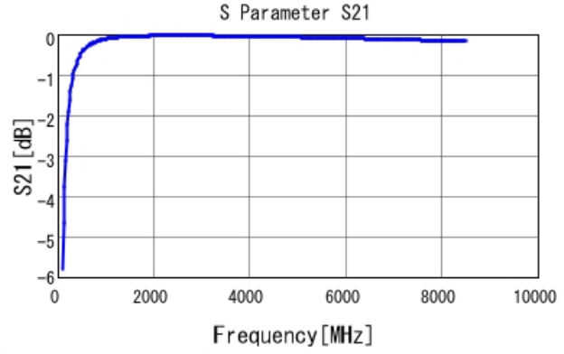
GRM0335C1H9R5CA01 S21 DC0V, 25degC
