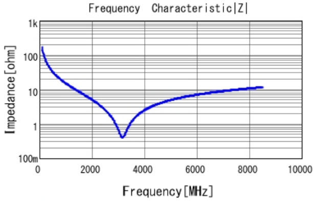
GRM0335C1H9R5CA01 |Z| DCOV, 25degC
