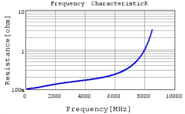
GQM1555C2D4R3BB01 R DC0V, 25degC
