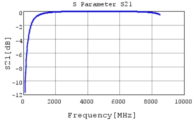
GQM1555C2D4R3BB01 S21 DCOV, 25degC
