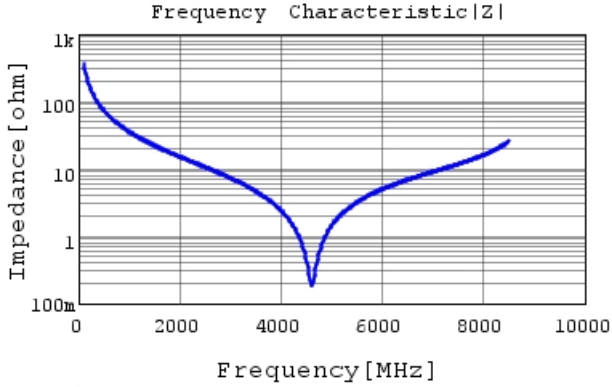
GQM1555C2D4R3BB01 |Z| DC0V, 25degC
