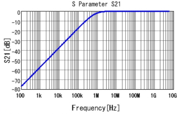
■ GCE188R72A222KA01 S21 DCOV, 25degC
