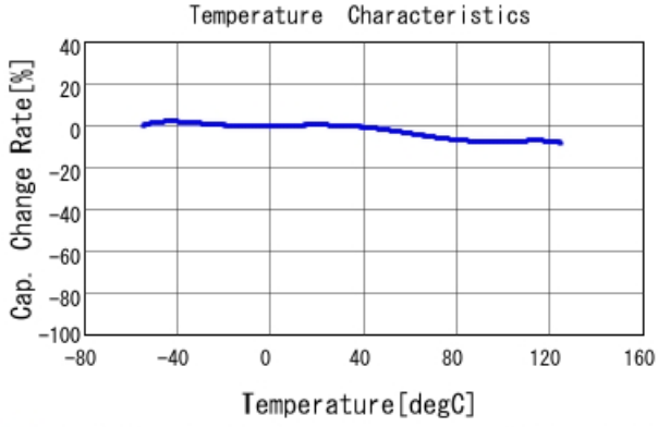
■ GCE188R72A222KA01 C-Temp. capchange, DCO. 0V, AC1. 0Vrm
