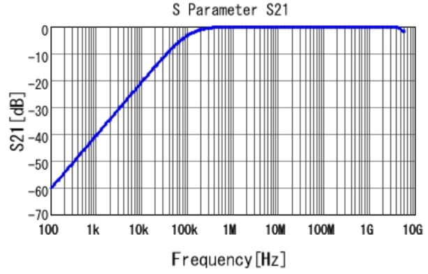
■ GCD188R72A153MA01 S21 DCOV, 25degC
