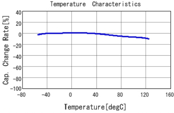
■ GCD188R72A153MA01 C-Temp. capchange, DCO. 0V, AC1. 0Vrm
