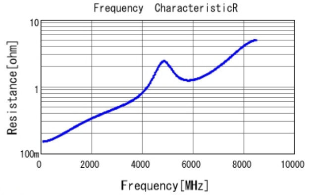
■ GRT1555C1H150JA02 R DC0V, 25degC
