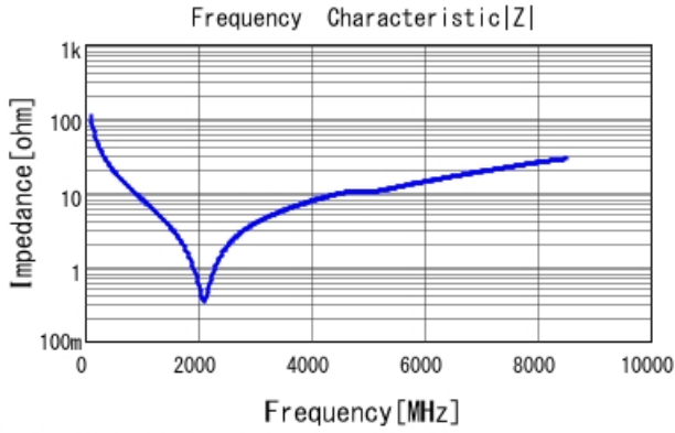
■ GRT1555C1H150JA02 |Z| DC0V, 25degC
