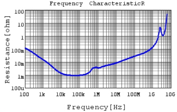
GRM32EC80E227ME05 R DCOV, 25degC
