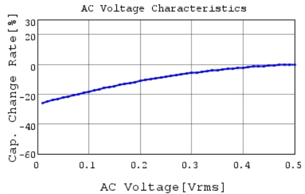
GRM32EC80E227ME05 C-AC Voltage capchange, Dc
