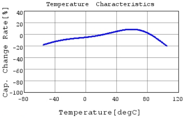
GRM32EC80E227ME05 C-Temp. capchange, DC0.0V,
