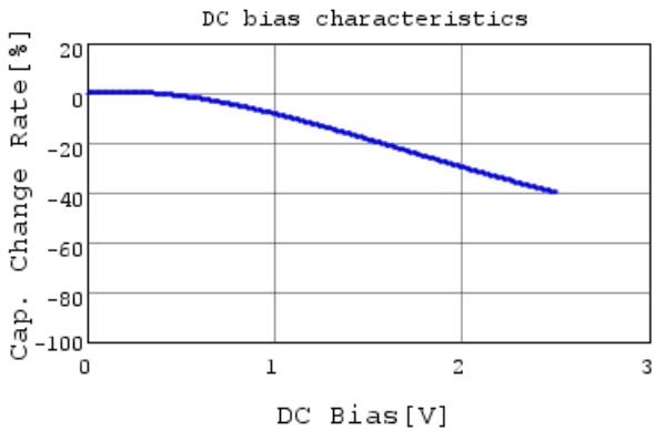
GRM32EC80E227ME05 C-DC bias capchange, 25.0c
