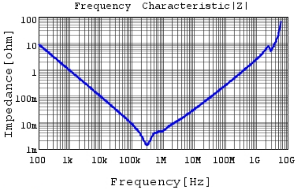
GRM32EC80E227ME05 |Z| DCOV, 25degC
