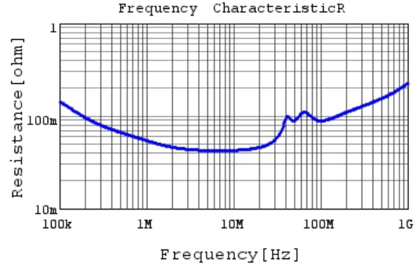
RCER72A104K1K1H03B R DCOV, 25degC
