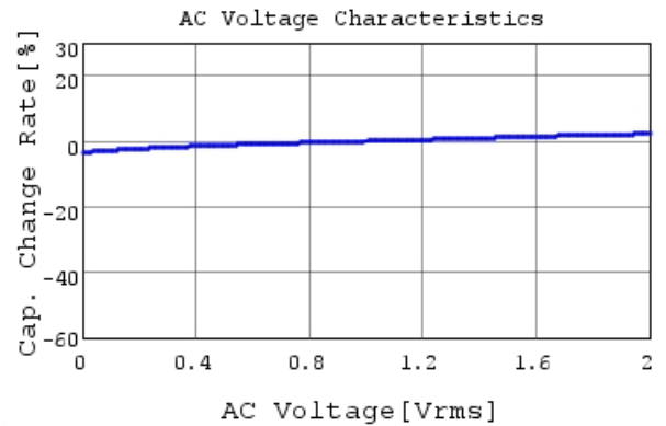
RCER72A104K1K1H03B C-AC Voltage capchange, I
