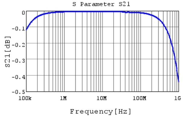
RCER72A104K1K1H03B S21 DC0V, 25degC
