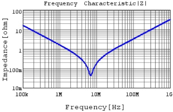
RCER72A104K1K1H03B |Z| DCOV, 25degC
