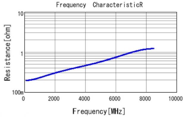
GRM0335C1H7R2BA01 R DCOV, 25degC
