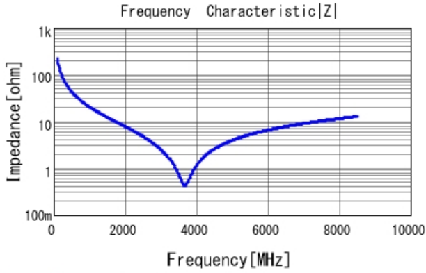
GRM0335C1H7R2BA01 |Z| DCOV, 25degC
