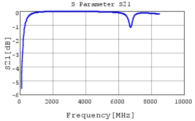
GCQ1555C1H9R9DB01 S21 DCOV, 25degC
