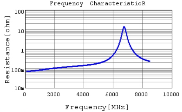
GCQ1555C1H9R9DB01 R DC0V, 25degC
