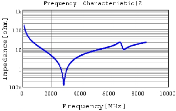
GCQ1555C1H9R9DB01 |Z| DC0V, 25degC
