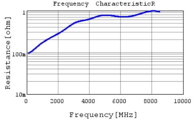
GRM0225C1E121JA02 R DCOV, 25degC
