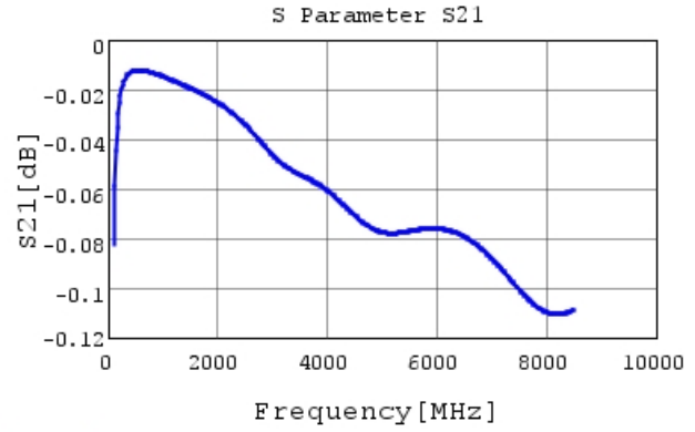
GRM0225C1E121JA02 S21 DCOV, 25degC
