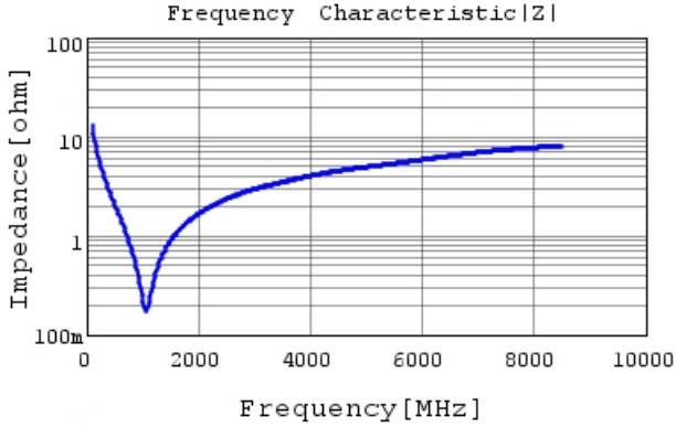
GRM0225C1E121JA02 |Z| DCOV, 25degC
