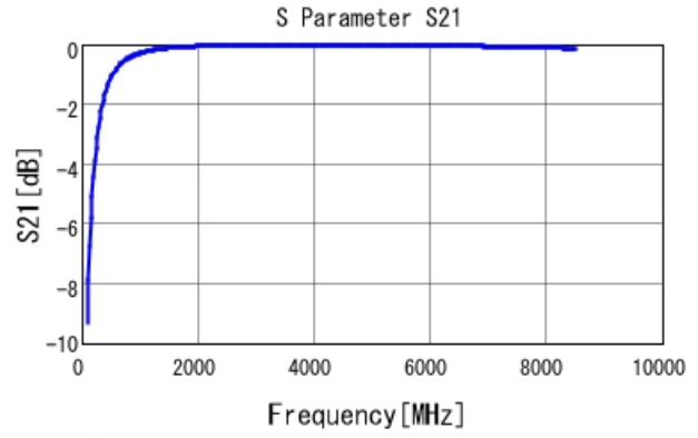
GJM0335C1E5R8BB01 S21 DC0V, 25degC
