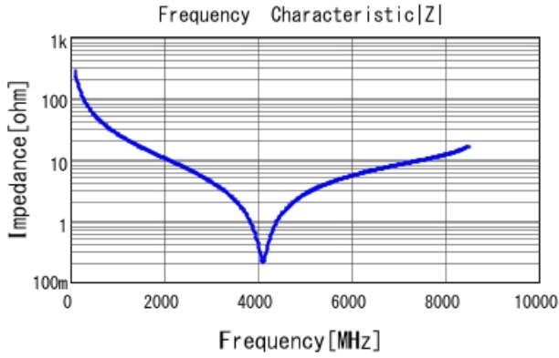
GJM0335C1E5R8BB01 |Z| DC0V, 25degC
