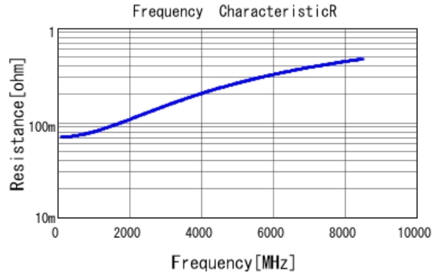
GJM0335C1E5R8BB01 R DC0V, 25degC
