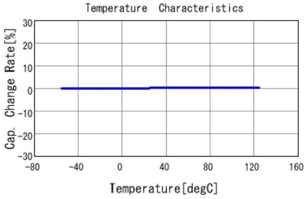
GJM0335C1E5R8BB01 C-Temp. capchange, DC0V, AC1Vrms
