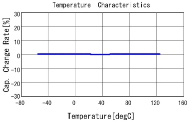
GCM2195C1K822JA16 C-Temp. capchange, DCOV, AC1Vrms
