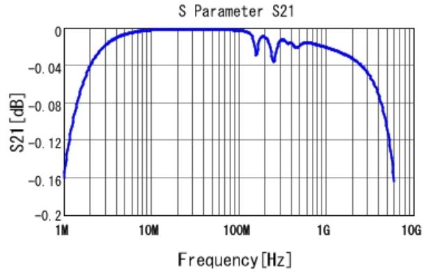
GCM2195C1K822JA16 S21 DCOV, 25degC
