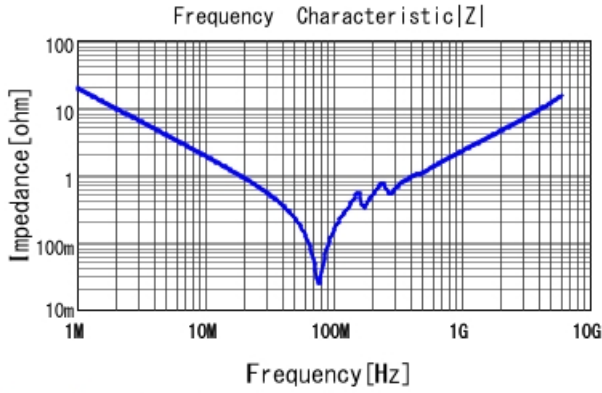
GCM2195C1K822JA16 |Z| DCOV, 25degC
