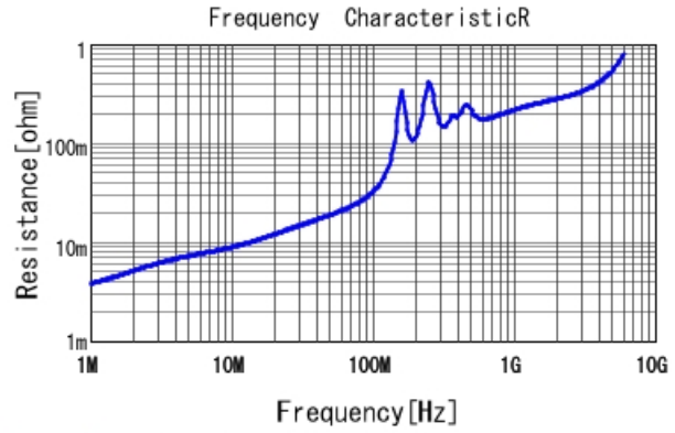
GCM2195C1K822JA16 R DCOV, 25degC
