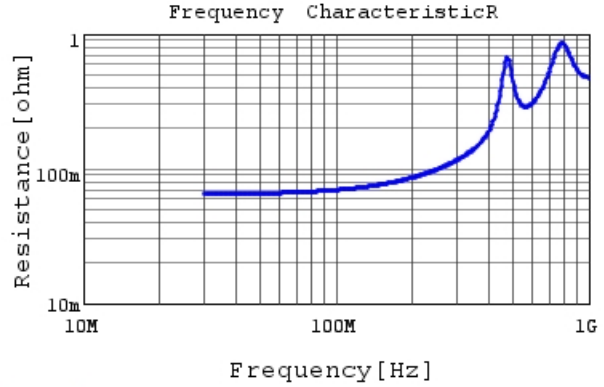
RCE5C1H821J0K1H03B R DC0V, 25degC
