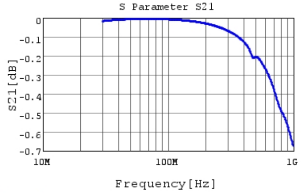
RCE5C1H821J0K1H03B S21 DCOV, 25degC
