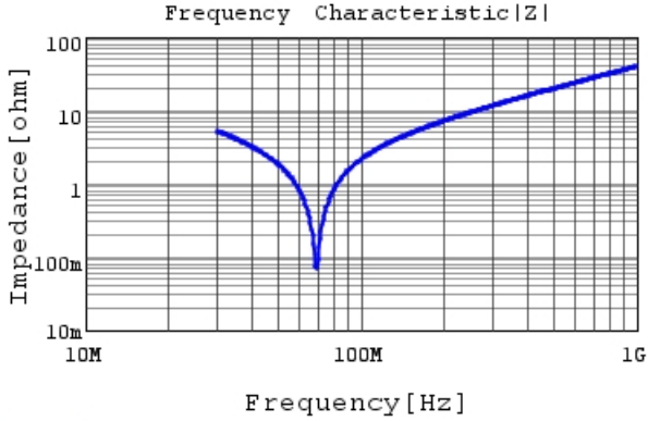
RCE5C1H821J0K1H03B |Z| DC0V, 25degC
