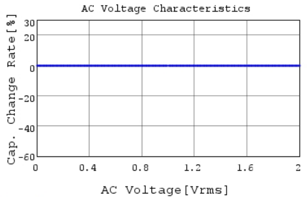
RCE5C1H821J0K1H03B C-AC Voltage capchange, I
