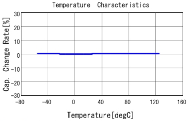
GQM1875C2E2R0CB12 C-Temp. capchange, DCOV, AC1Vrms
