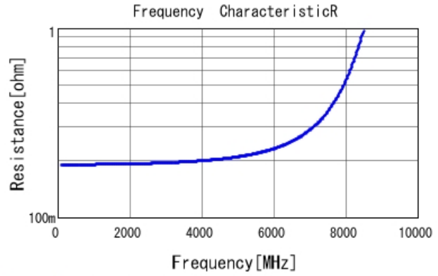
GQM1875C2E2R0CB12 R DCOV, 25degC
