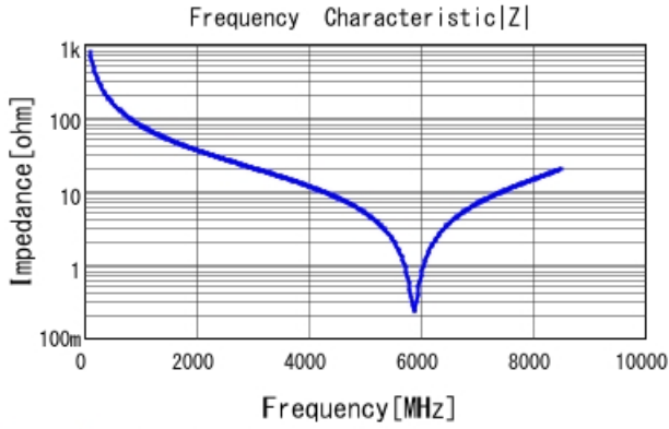
GQM1875C2E2R0CB12 |Z| DCOV, 25degC
