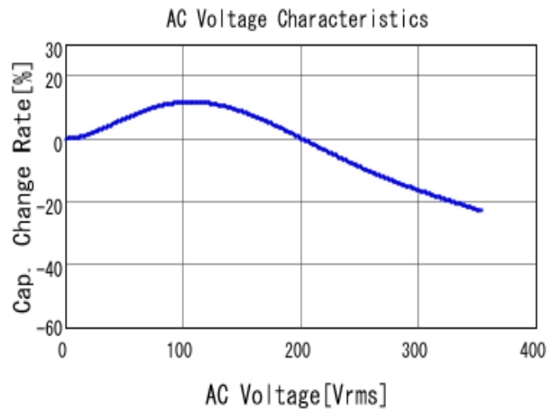
■ GRJ32DR73A223KWJ1 C-AC Voltage capchange, DCOV, 25.0d
