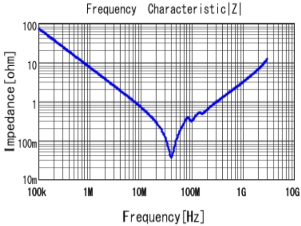
■ GRJ32DR73A223KWJ1 |Z| DCOV, 25degC
