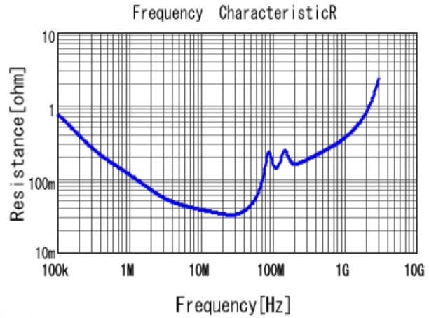
■ GRJ32DR73A223KWJ1 R DCOV, 25degC
