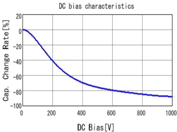
■ GRJ32DR73A223KWJ1 C-DC bias capchange, 25.0degC, AC1V
