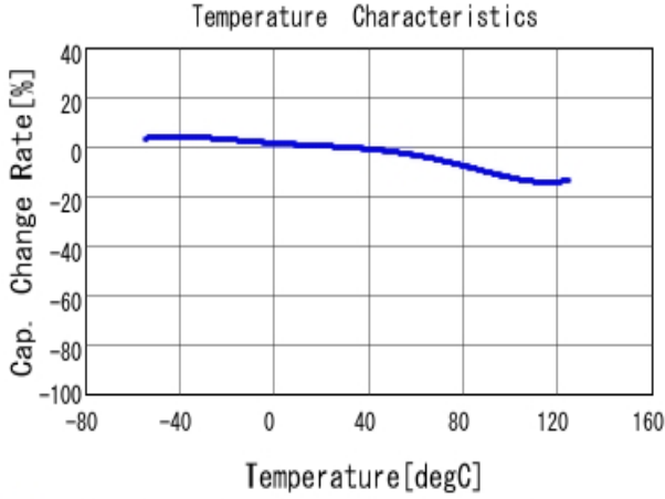
■ GRJ32DR73A223KWJ1 C-Temp. capchange, DCOV, AC1Vrms
