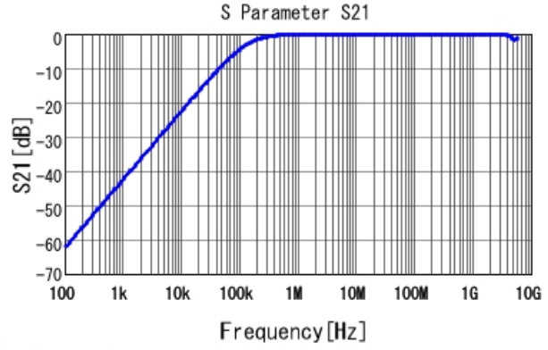
■ GCD188R72A123MA01 S21 DCOV, 25degC
