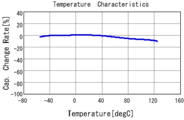
■ GCD188R72A123MA01 C-Temp. capchange, DCO. 0V, AC1. 0Vrm
