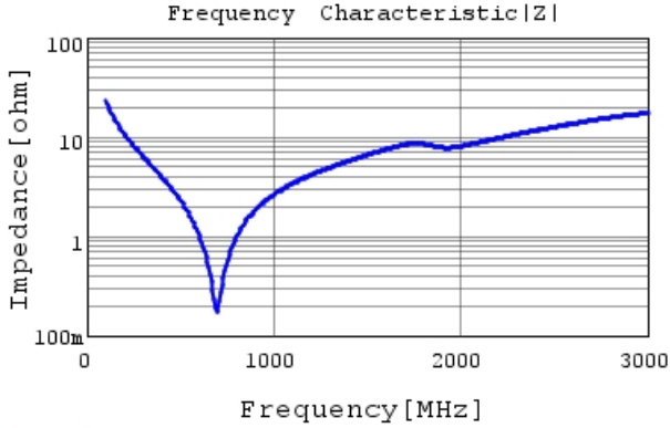
GRM31A7U3A680JW31 |Z| DC0V, 25degC
