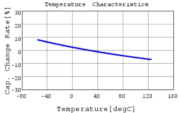
GRM31A7U3A680JW31 C-Temp. capchange, DC0V, 1
