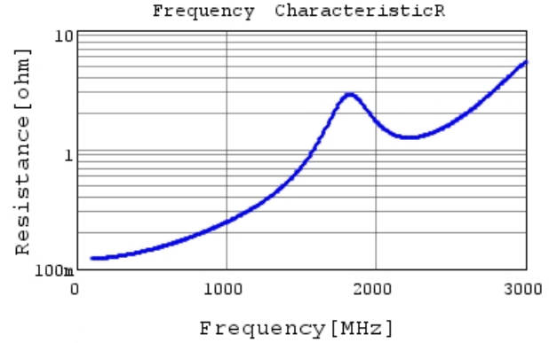
GRM31A7U3A680JW31 R DC0V, 25degC
